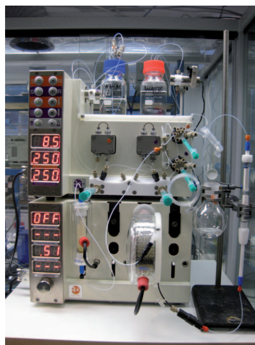
Figure 1. Vapourtec R2 + /R4 flow system.
